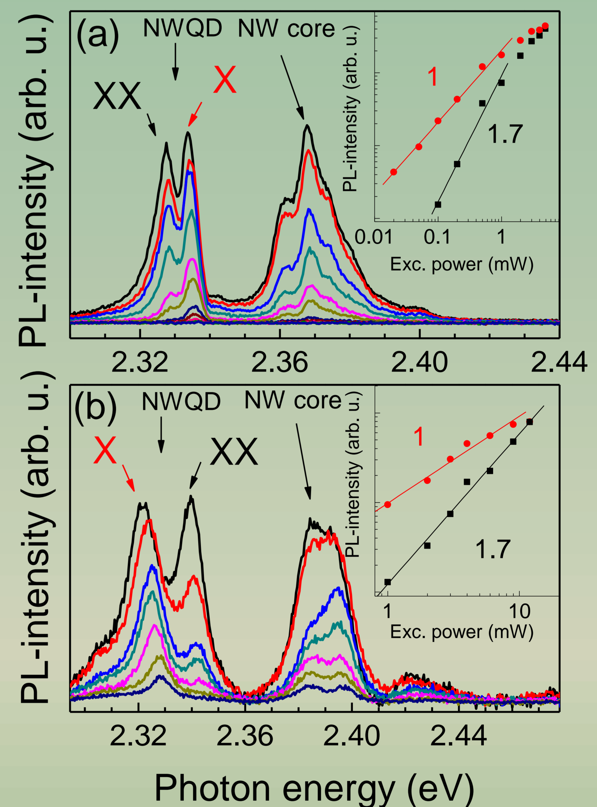
Fig. 4 \mu -PL spectra with increasing excitation fluence from relatively short (7nm) individual ZnTe/ZnMgTe NWQDs (a) and relatively long (45 nm) NWQDs (b). Biexciton binding energy exhibits either binding or antibinding character respectively. Temperature of measurements- 7 K, excitation- 405 nm.
