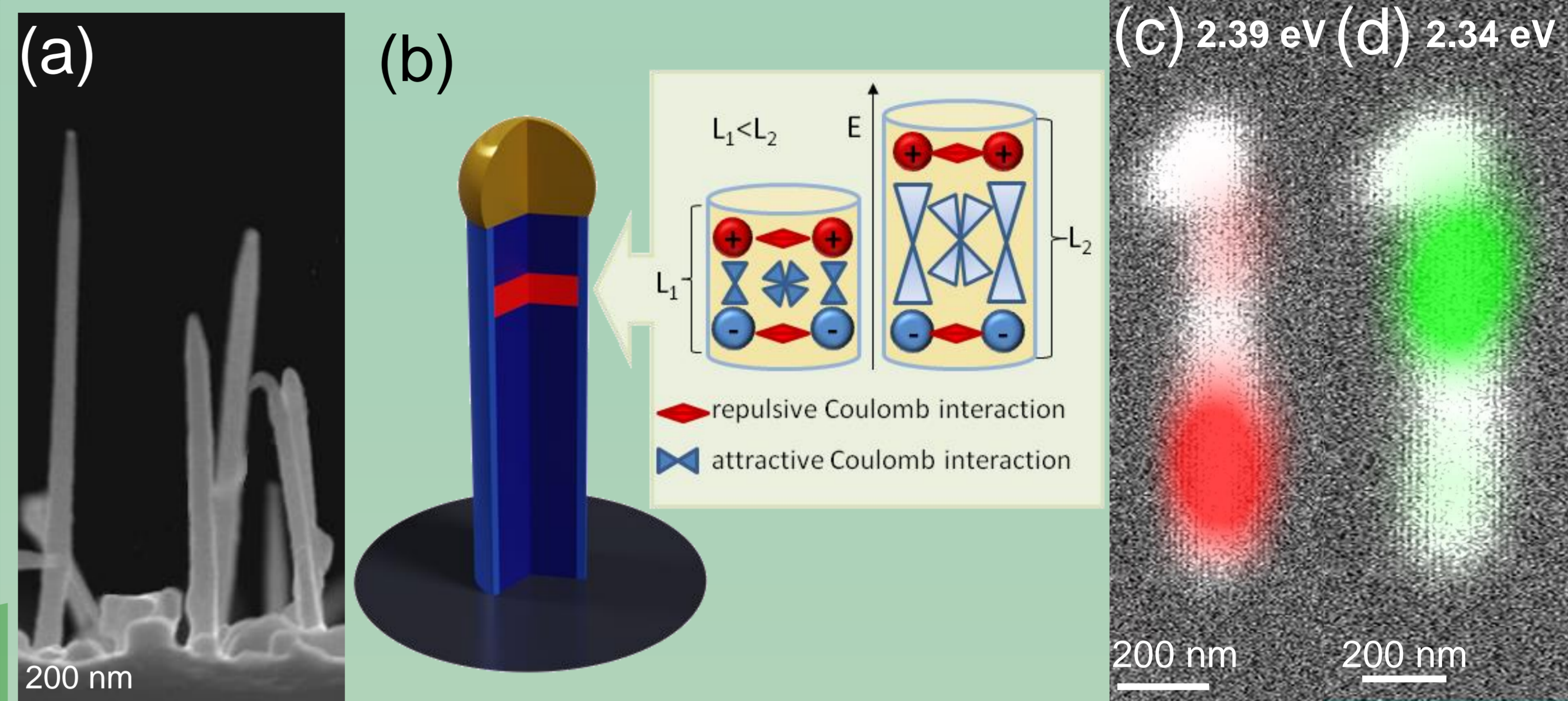
Fig. 2 (a) SEM image of investigated nanowires. (b) Scheme of investigated nanowire heterostructure along with schematic arrangement of electrons and holes inside ZnTe nanowire quantum dot and corresponding attractive (blue) and repulsive (red) interactions within biexciton complexes. In longer NWQDs the attractive Coulomb interaction is reduced. (c)(d) Cathodoluminescence map performed at 2.39 eV – nanowire core (c) and 2.34 eV – NWQD (d) combined with SEM image. Probe current is set to 500 pA, acceleration voltage is set to 15 kV and temperature is stabilized at 7 K.
